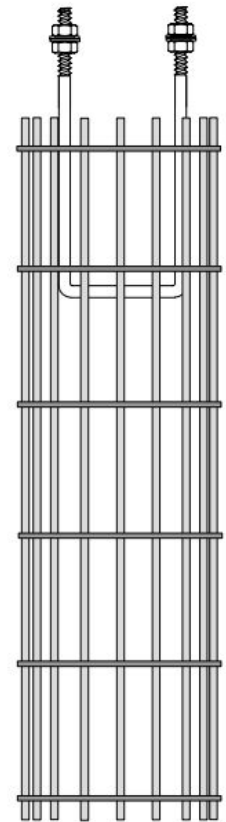
Typical Footing Cage Layout
